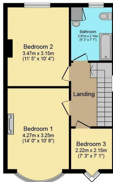
First Floor Floor area 48.4 sq.m. (521 sq.ft.) approx
