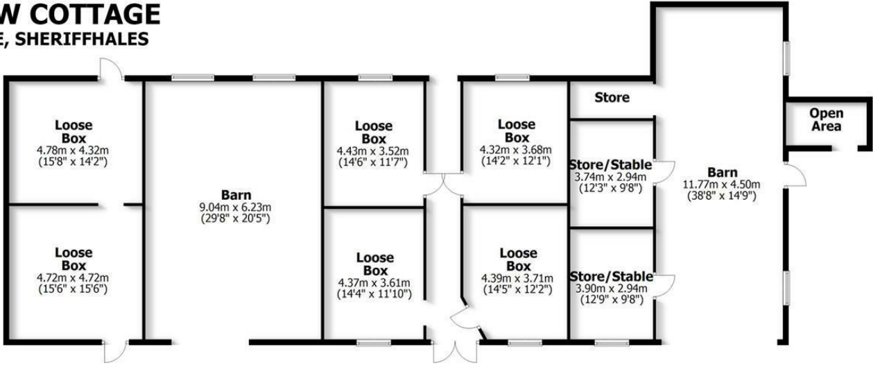
Outbuilding
