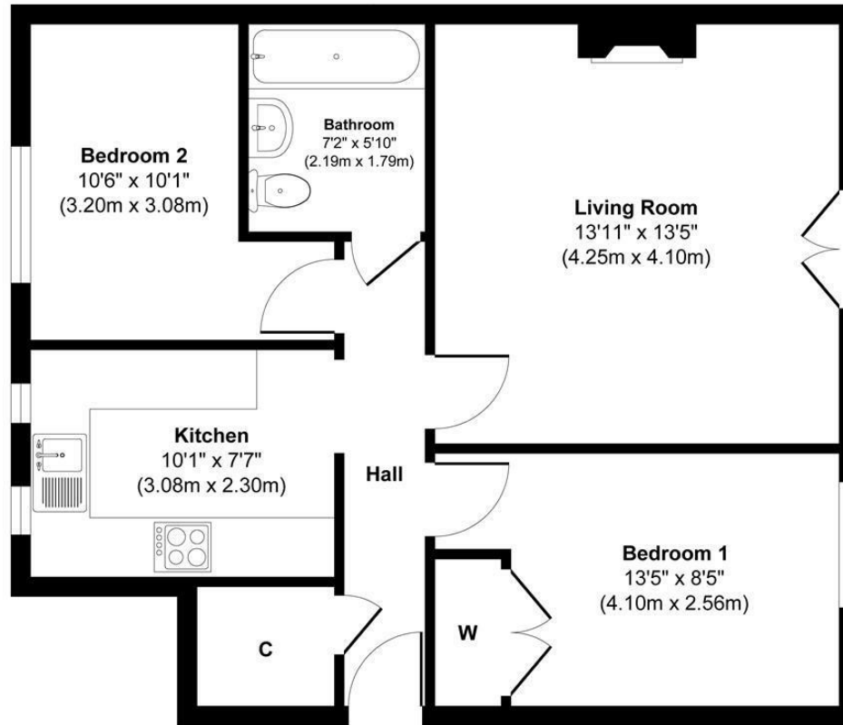
Floor Plan
