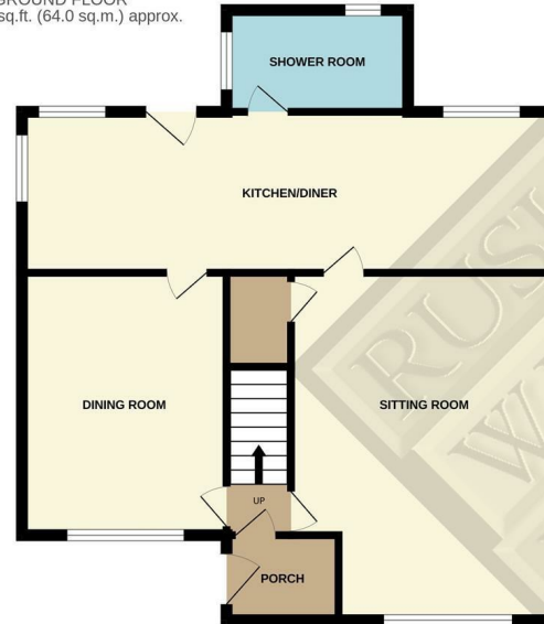
GROUND FLOOR 689 sq.ft. (64.0 sq.m.) approx.
