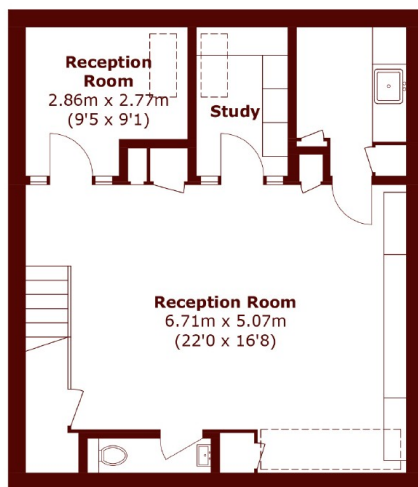
Basement
