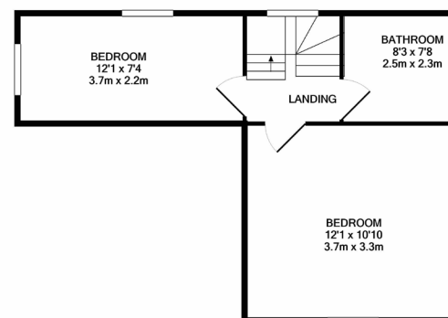
1ST FLOOR APPROX. FLOOR AREA 576 SQ.FT. (53.5 SQ.M.)
