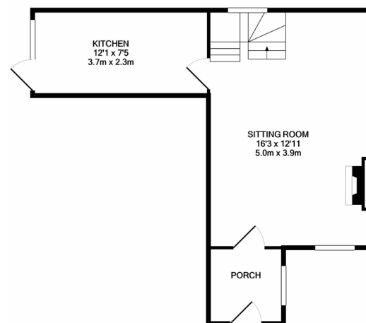
GROUND FLOOR APPROX. FLOOR AREA 635 SQ.FT. (59.0 SQ.M.)
