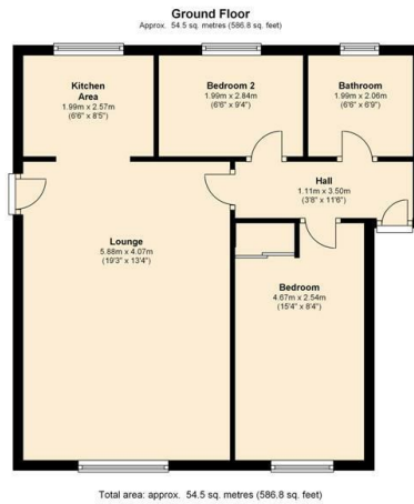
FLOOR PLAN - Flat 1 Quercus Court, Oakthorpe Road, OX2 7BF
