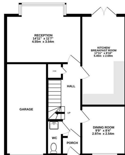
GROUND FLOOR 676 sq.ft. (62.8 sq.m.) approx.
