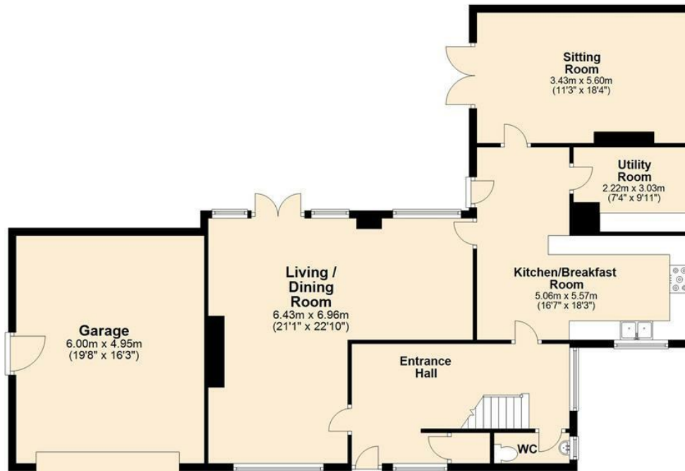
Ground Floor Approx. 131.0 sq. metres (1409.8 sq. feet)
