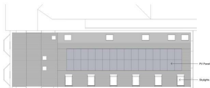
Proposed Roof 1 : 100
