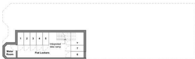
Proposed Basement 1 : 100
