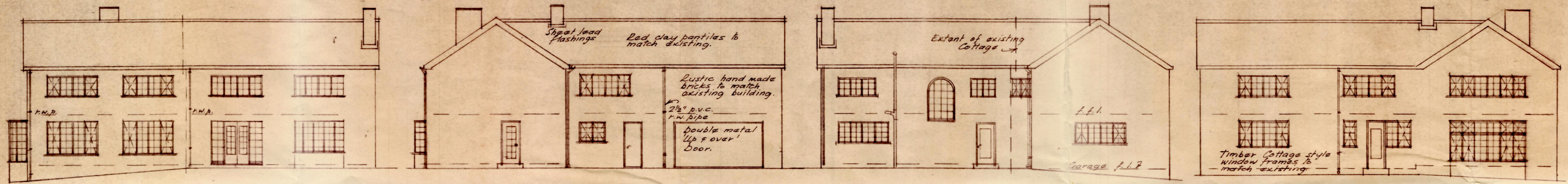
SOUTH ELEVATION
