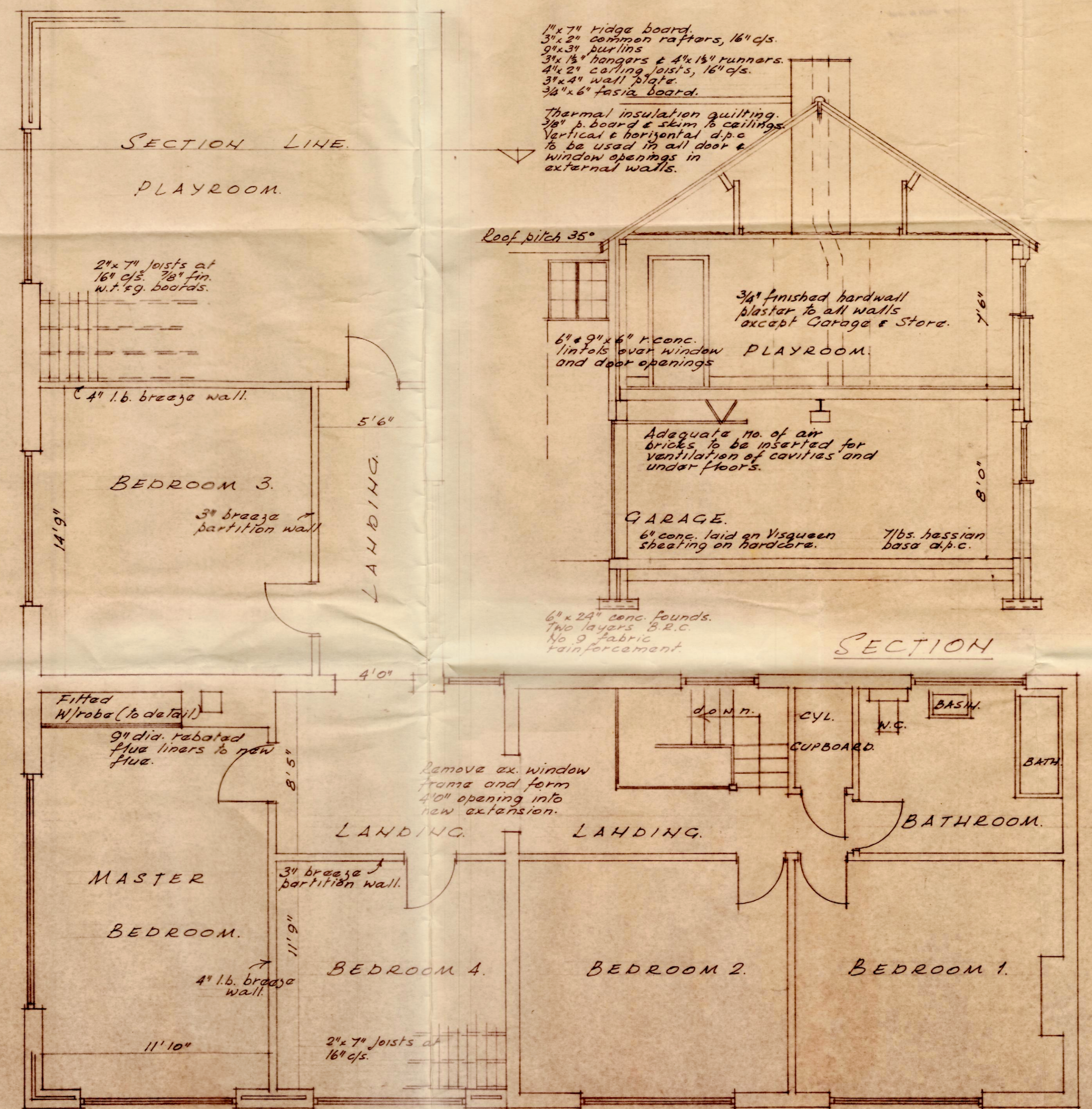
FIRST FLOOR.
