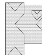
1.2 PROPOSED ROOF LAYOUT SCALE: 1:100 @ A1
