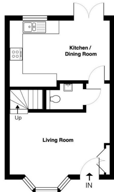
Plot 9, 8 Oast Gardens Approx Internal Area 778 sq ft (72.3 sq m)
