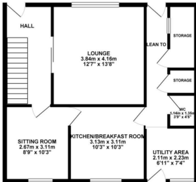
GROUND FLOOR 57.52 sq. m. ( 619.16 sq. ft. )
