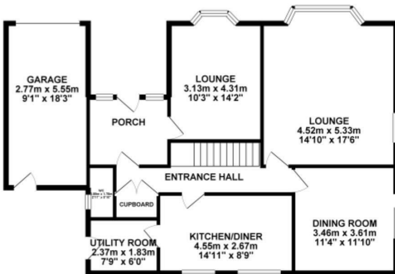
GROUND FLOOR 97.70 sq. m. ( 1051.61 sq. ft. )
