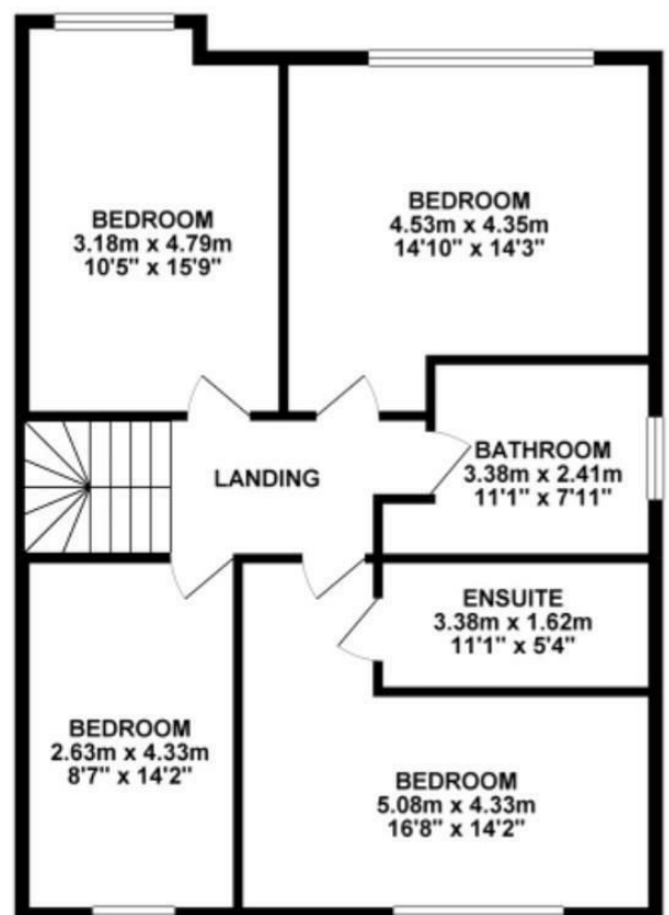
1ST FLOOR 81.16 sq. m. ( 873.56 sq. ft. )
