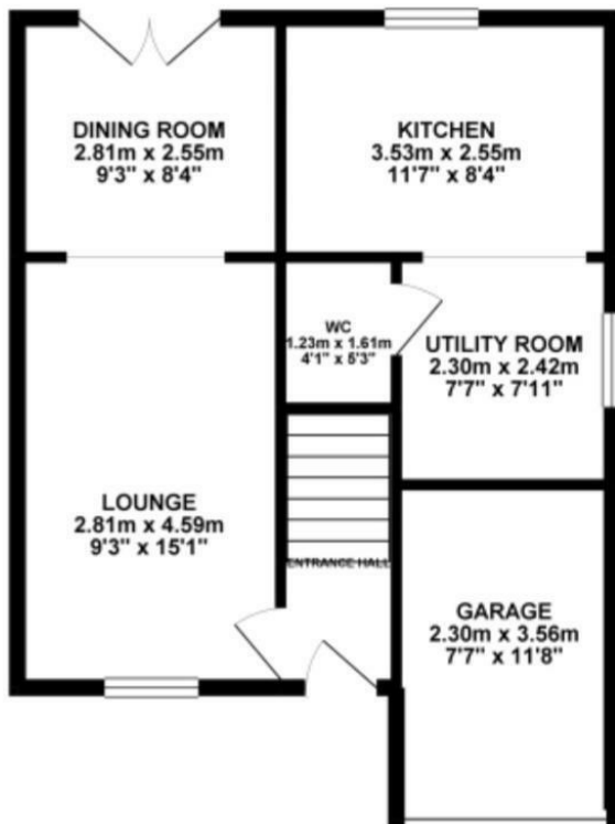
GROUND FLOOR 48.46 sq. m. ( 521.57 sq. ft. )
