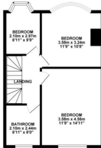
1ST FLOOR 45.48 sq. m. ( 489.51 sq. ft. )
