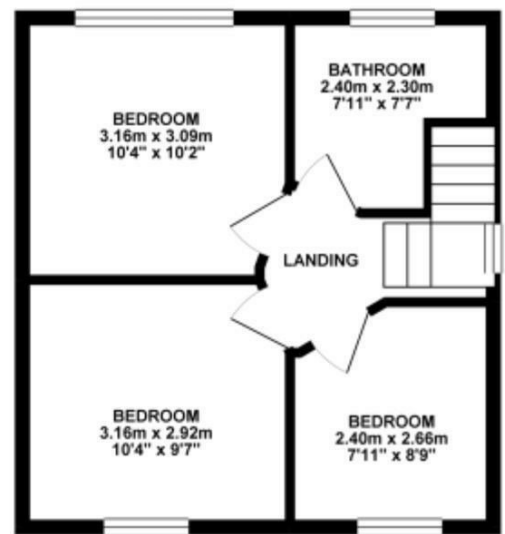
1ST FLOOR 33.46 sq. m. ( 360.12 sq. ft. )
