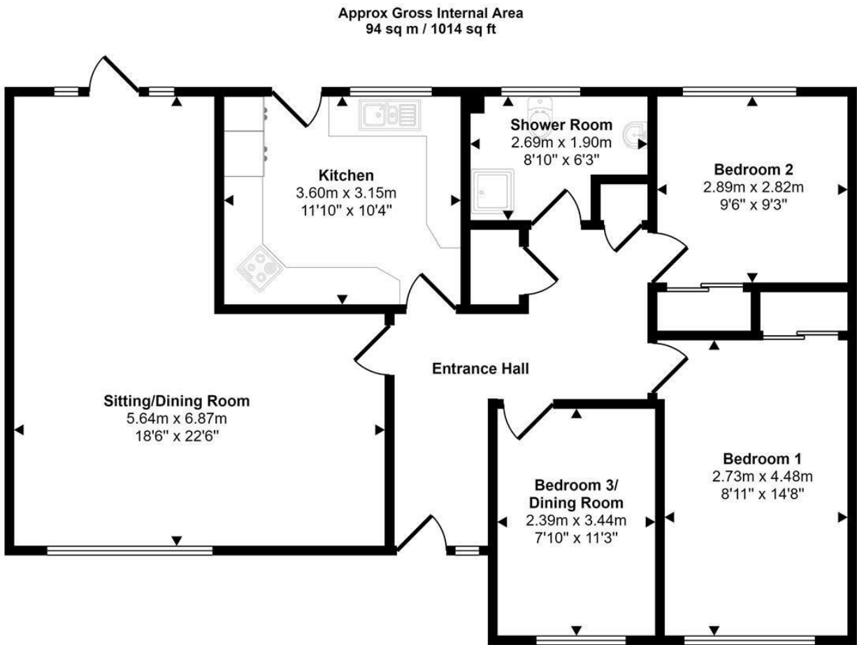
Floorplan
