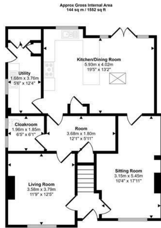
Ground Floor Approx 80 sq m / 865 sq ft
