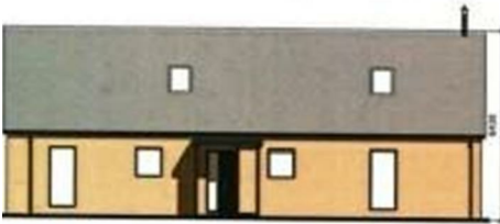
Front Elevation 1:100
