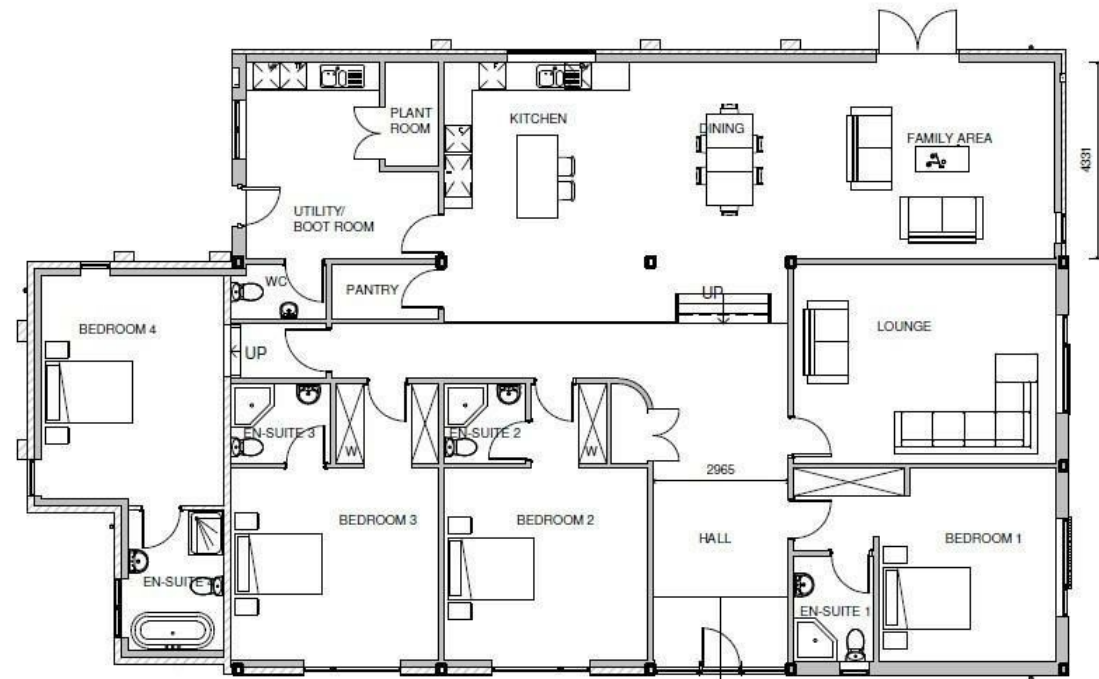
Proposed Floorplan
