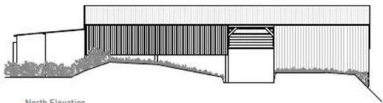
North Elevation 1:100
