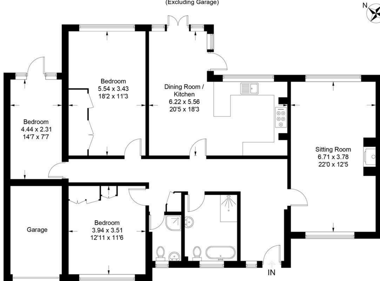
Ground Floor
