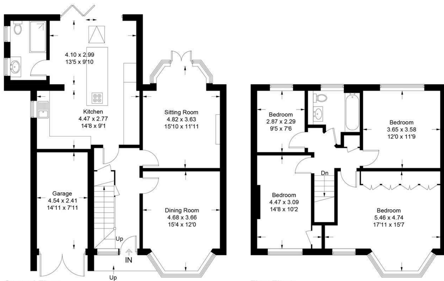
Ground Floor
