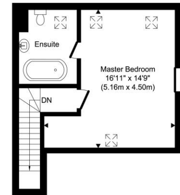
Second Floor Approximate Floor Area 339.60 sq. ft. (31.55 sq. m)
