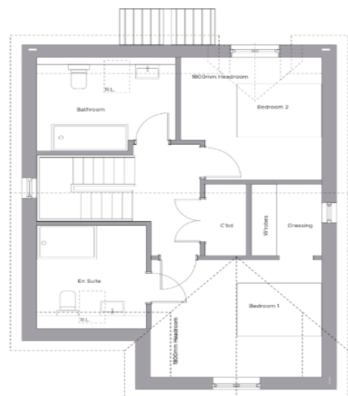
FIRST FLOOR PLAN Scale: 1:50
