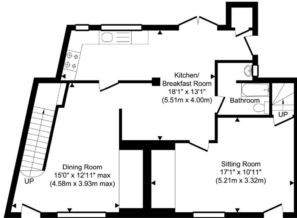
Ground Floor Approximate Floor Area 645.83 sq. ft. (60.00 sq. m)
