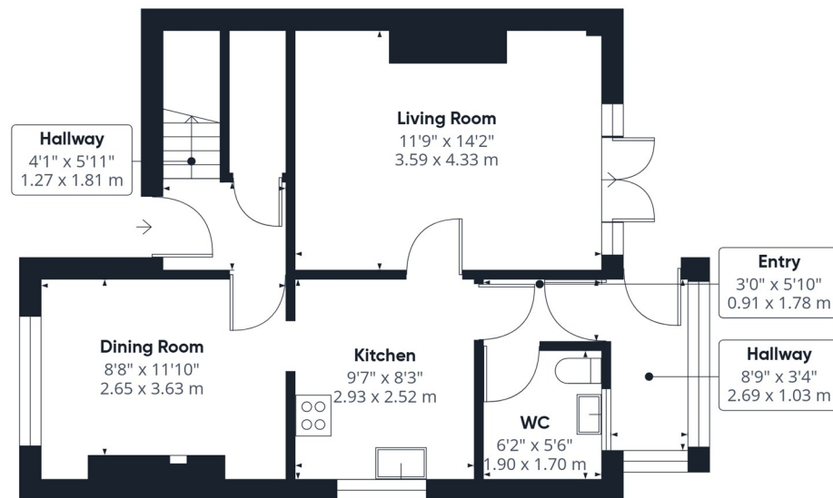
Floor 0 Building 1
