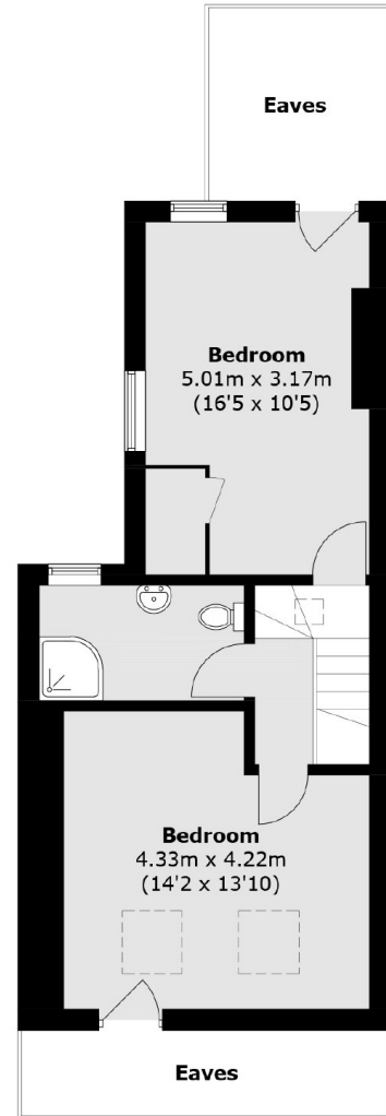
Second Floor
