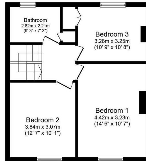
First Floor Floor area 45.3 sq.m. (488 sq.ft.)
