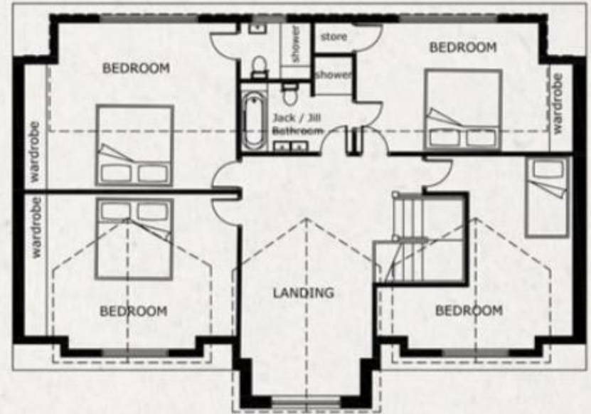
PROPOSED FIRST FLOOR PLAN SCALE 1:100
