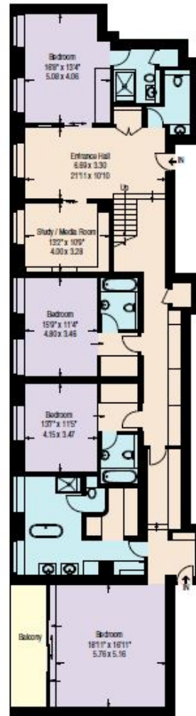
Fifteenth Floor
