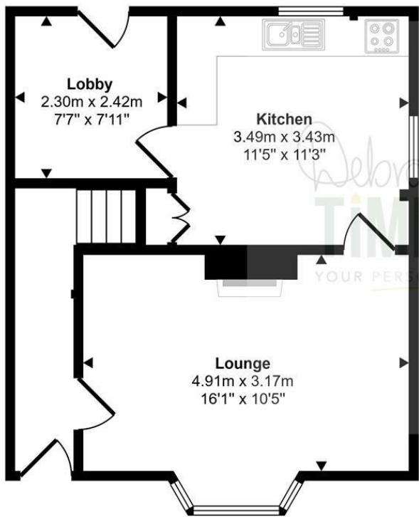
Ground Floor Approx 41 sq m / 444 sq ft
