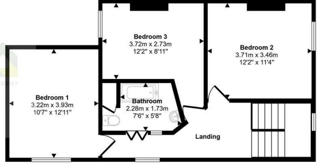
First Floor Approx 56 sq m / 599 sq ft
