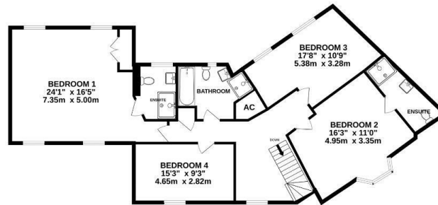
1ST FLOOR
