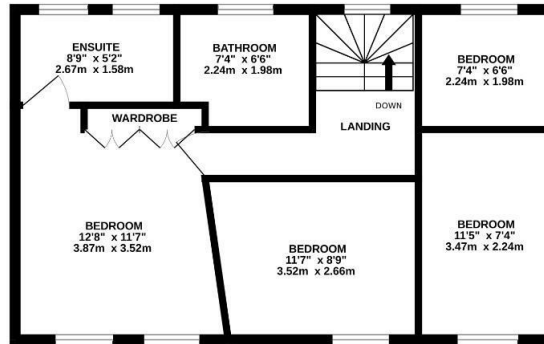
1ST FLOOR 522 sq.ft. (48.5 sq.m.) approx.
