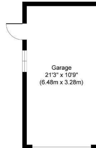
Garage Approximate Floor Area 228 sq. ft (21.22 sq. m)
