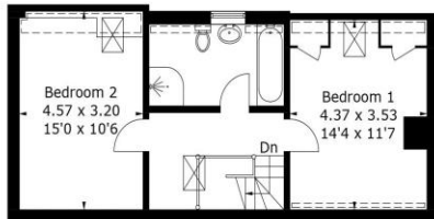
Outbuilding - First Floor
