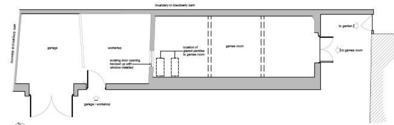
Existing Ground Floor Plan 1:100 Scale
