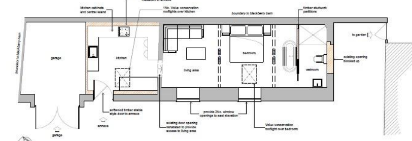
Proposed Ground Floor Plan 1:100 Scale
