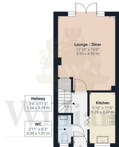
Floor 0
