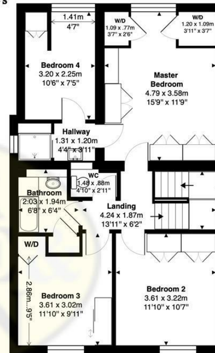
First Floor Floor Area: 67.6 m 2 ... 728 ft 2
