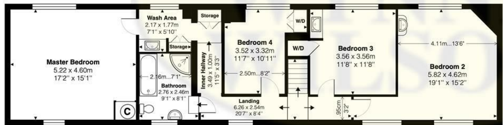
First Floor Floor Area: 93.3 m 2 ... 1004 ft 2
