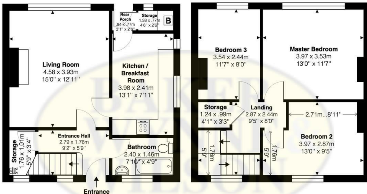
Ground Floor Floor Area: 41.8 m 2 ... 450 ft 2
