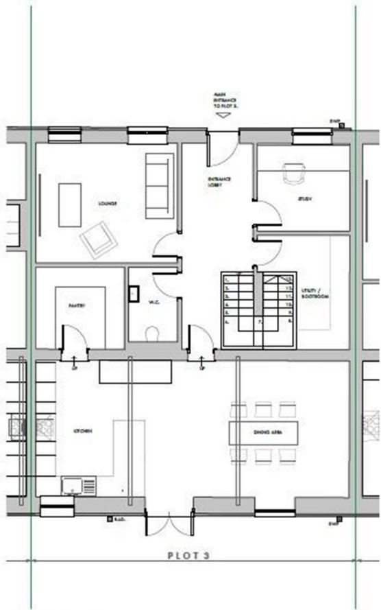
GROUND FLOOR PLAN PLOT 3
