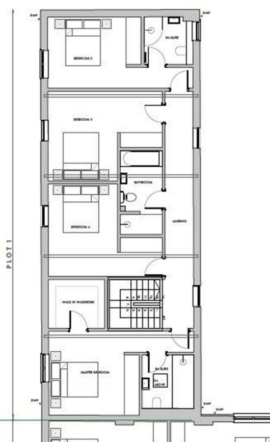
FIRST FLOOR PLAN PLOT 1
