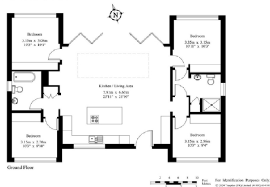
The Horseshoes Annexe Gross Internal Area : 110.3 sq.m (1187 sq.ft.)
