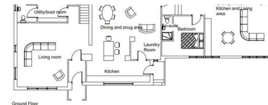
PROPOSED FLOOR PLANS - OPTION 1 SCALE: 1:100@A1
