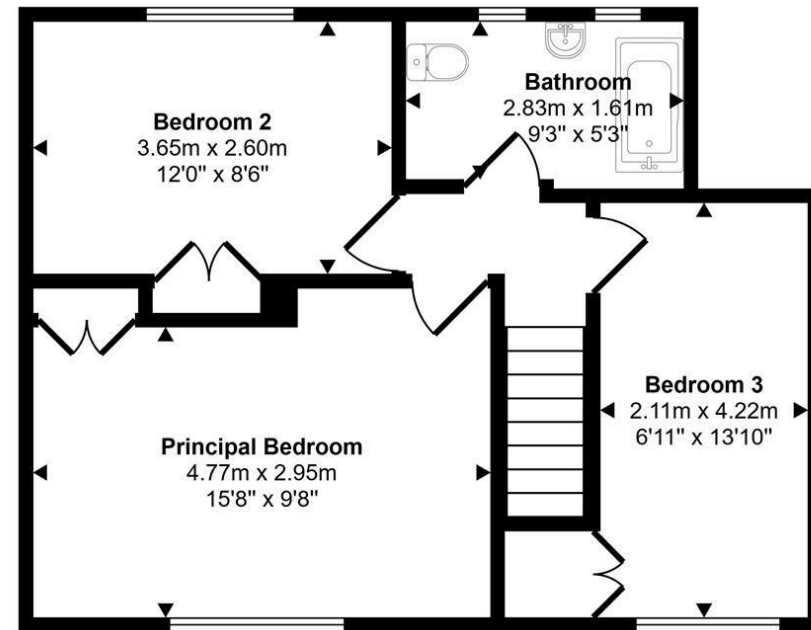
First Floor Approx 46 sq m / 494 sq ft
