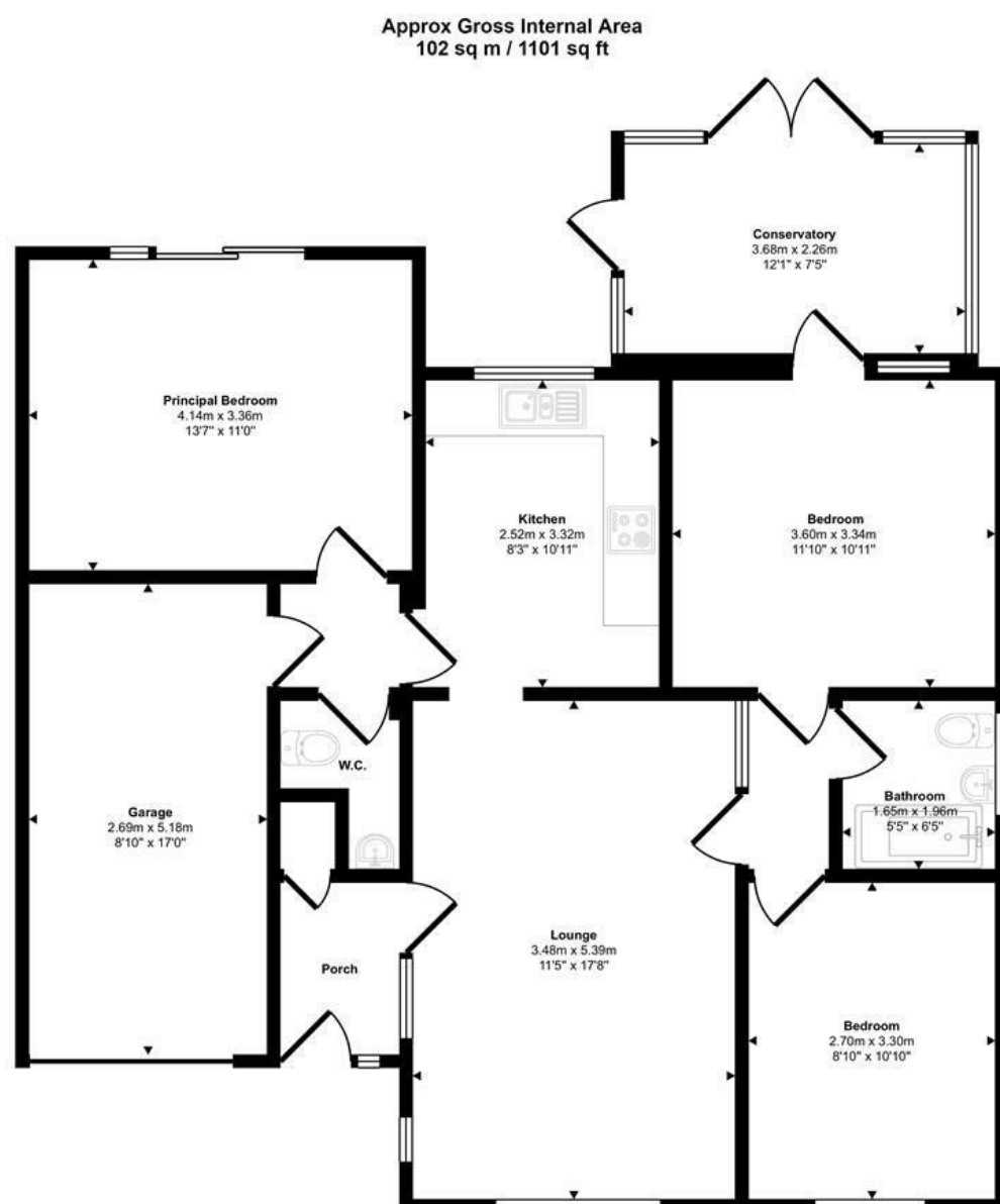
Floorplan
